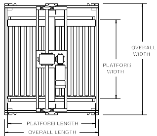
RVC TOP VIEW
