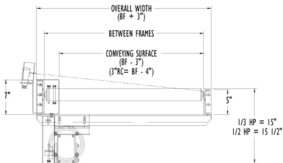
SZD25 ICDA UNDERNEATH DRIVE
