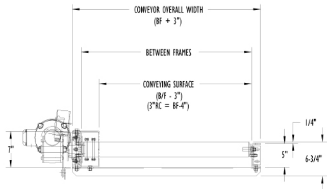
SZD25 ICDA SIDEMOUNT DRIVE
