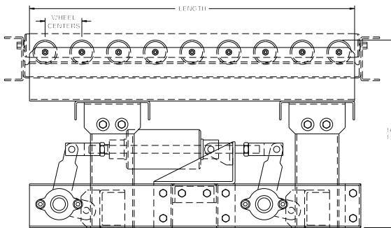
Shown mounted in optional conveyor
